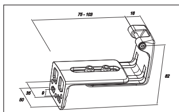
Aluminium adjustable "Z" bracket for bottom hinged window
