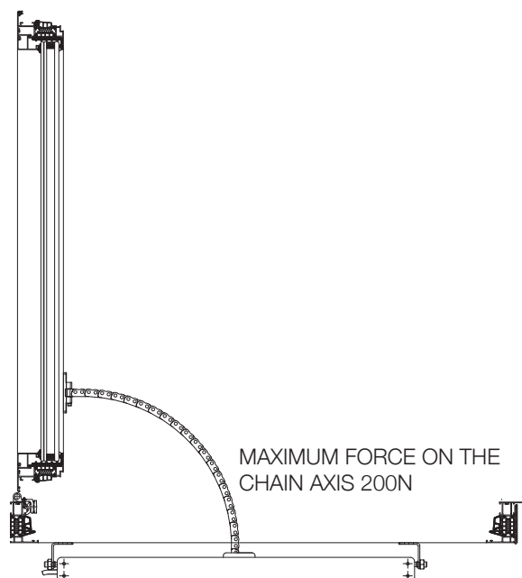
Side hinged window opening inward.
