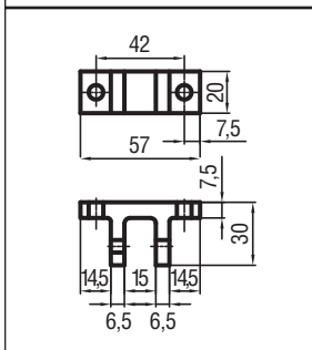
Aluminium back bracket part No. 35697P
