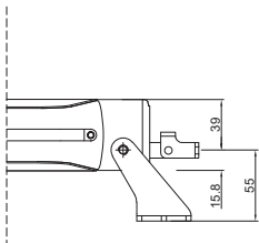
T-Rack actuator with end bracket part No. 41760Y
