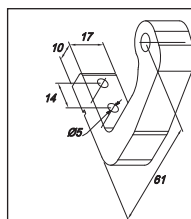
"C" pivoting brackets for bottom hinged windows (to be ordered separately):
